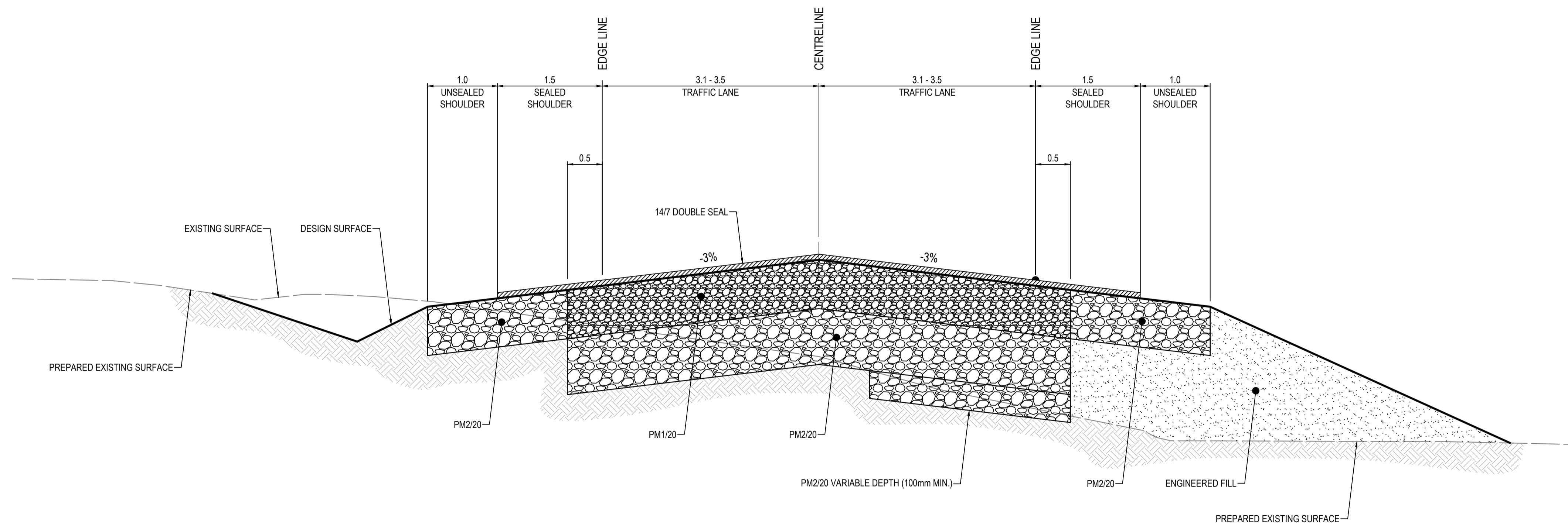
TYPICAL RURAL PAVEMENT CROSS SECTION
