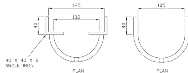
CHANNEL MOUNTED BRACKET 6310 - 0070
