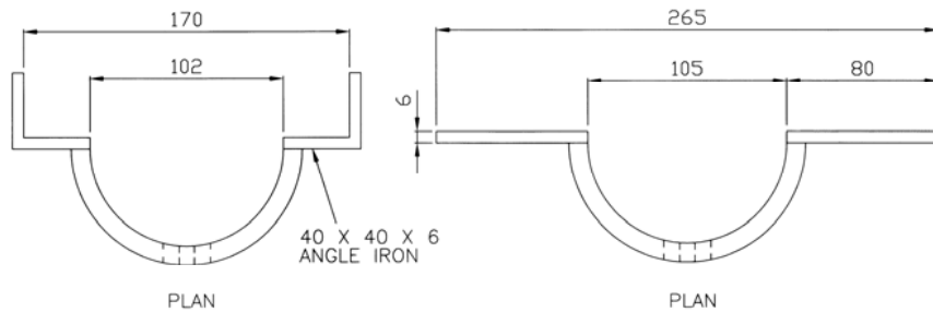
CHANNEL MOUNTED BRACKET 6310 - 0069
