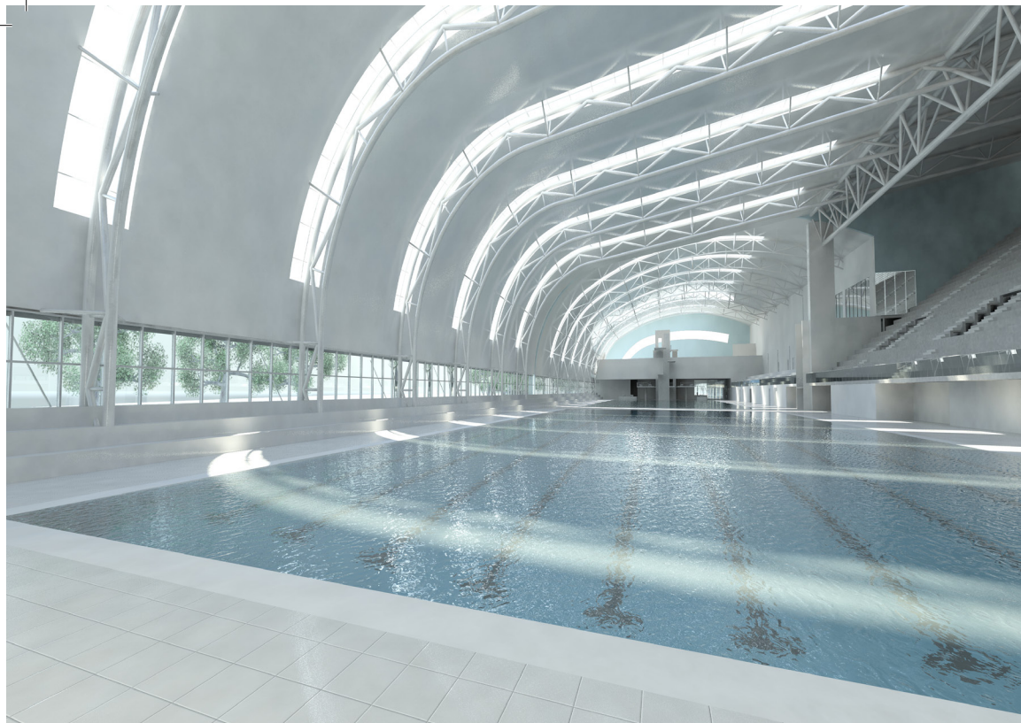
State Aquatic Centre Pool
